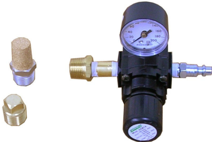
DD/DB Stand Mount Air Kit Part# 02568
